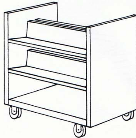
No. BT-45 – BOOK TRUCK – 4 sloping shelves with back, four 4" rubber swivel casters, can also be used for movable displays, size same as No. BT-40. 11" between shelves, 13½" from front of bottom shelf to base.
