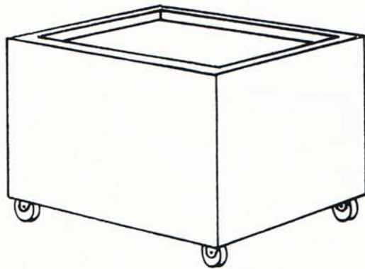
No. DBT-35 – DEPRESSABLE BOOK TRUCK – platform recedes as books are placed on it. Fits under standard desk or in corners for handy return of books. 28" high, 24½" wide, 20¾" deep with 4 swivel casters.
