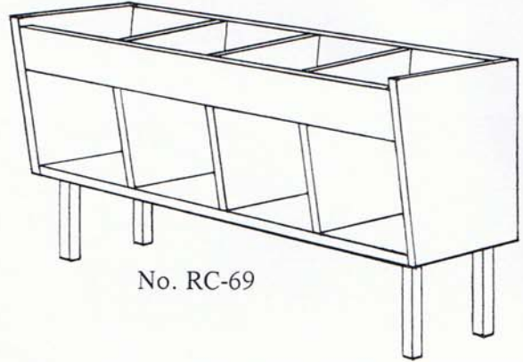
No. RC-69 – RECORD RACK – Holds 50 records per opening. 39" high, 19½" deep, 56" long. Top compartments 8¼" deep at back, 6¾" at front, 13" wide. Lower storage area 13" x 14½" high.
