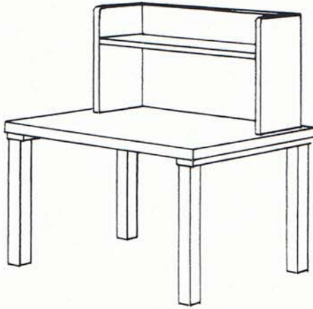
No. ST-22 – CARRELL TABLE – High back, 1½" desk top, 36" long, 24" deep, 29" from floor. Book shelf 8" deep, back 22" high from table top.
