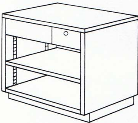
No. LCC-2 — CASH DRAWER UNIT — has solid top with two drawers under — 1 for cash with lock and 1 adjustable shelf.
